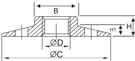
Clamping Nut
